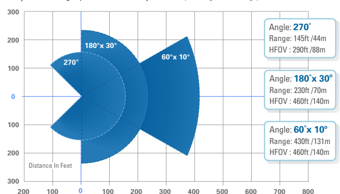
Options 2: Light panels rotated fully outward (max angle = min range)*
